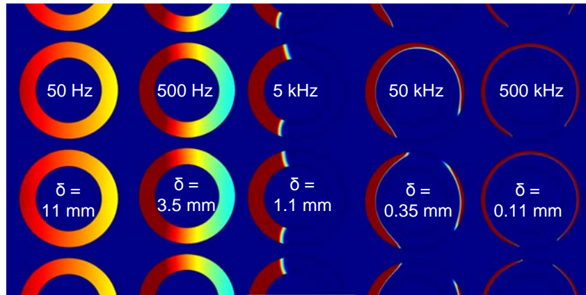
Figure 3. COMSOL® Results Showing Relative Current Distribution for Frequencies Ranging from 50 Hz to 500 kHz, (The Coil Centre Line is on the Left Side of the Conductors).
