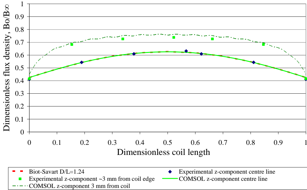
Figure 4. Dimensionless Magnetic Flux Density for a 16 Turn Induction Coil at 50 Hz, without a Work Piece.
