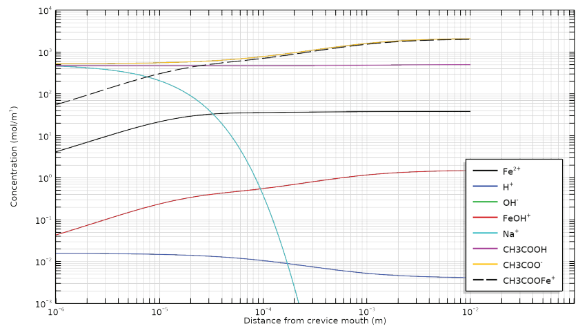
FIGURE 8. Concentration of ion and ion complexes along the depth of a crevice.
