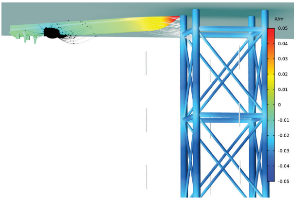
FIGURE 18. A boat anchored close to an oil rig is subjected to the currents from the cylindrical anodes that protect the rig structure from corrosion. The boat acts as a bipolar electrode, where parts of the hull close to the oil rig may corrode anodically. The black streamlines show the output from the ICCP anodes, and the gray streamlines show the direction of current toward the jacket structure.
