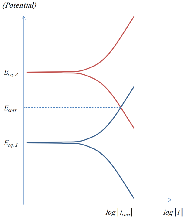
FIGURE 4. Evans diagram for two electrode reactions in the absence of ohmic and mass transport losses.
