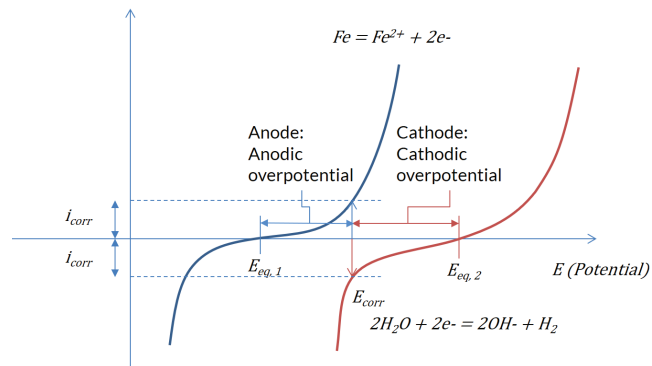
FIGURE 3. The Butler–Volmer expression for the reaction at the less noble metal surface (blue) and the more noble metal surface (red).
