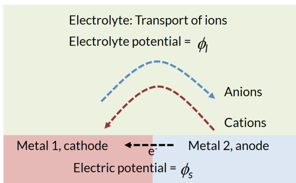
FIGURE 1. A galvanic cell where metal 1 acts as the cathode and metal 2 as the anode. The circuit is closed by the presence of an electrolyte, which covers both metal surfaces.
