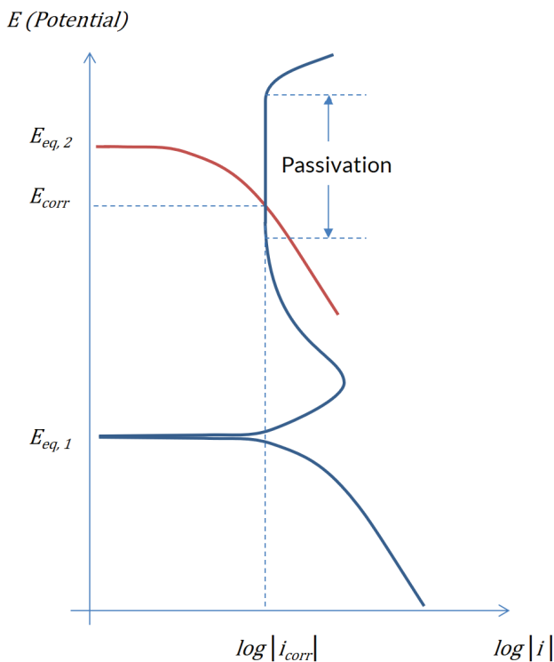
FIGURE 13. In anodic protection, the potential must be kept within the passivation window.
