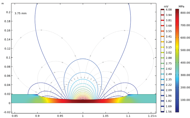
FIGURE 10. Stresses in a metal plate in contact with an electrolyte. The thinner region of the plate with the highest stresses acts as the anode.
