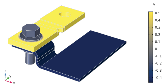
FIGURE 12. Electrode potential on the surface of a busbar assembly subjected to humid air. The structure is covered every now and then with a thin layer of condensed electrolyte. The simulation yields the corrosion rate of the different metals: copper (upper busbar), zinc (bolt), and aluminum (lower busbar).
