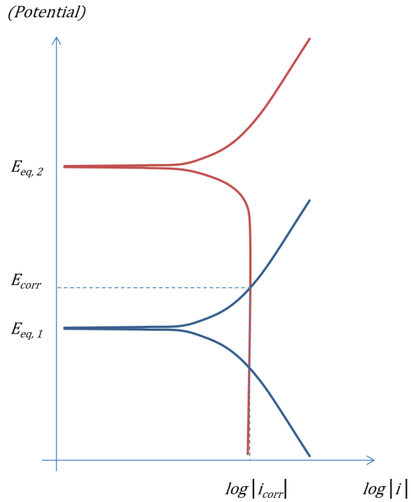
FIGURE 6. The Evans diagram for limiting current in the oxygen reduction reaction corresponding to the plot in Figure 5.
