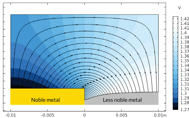
FIGURE 7. Streamlines of the current density and isopotential curves in the electrolyte in a galvanic cell. The initial surface of the noble metal and the less noble metal is horizontal at the initial state. After 72 h, the less noble metal is corroded through anodic dissolution.
