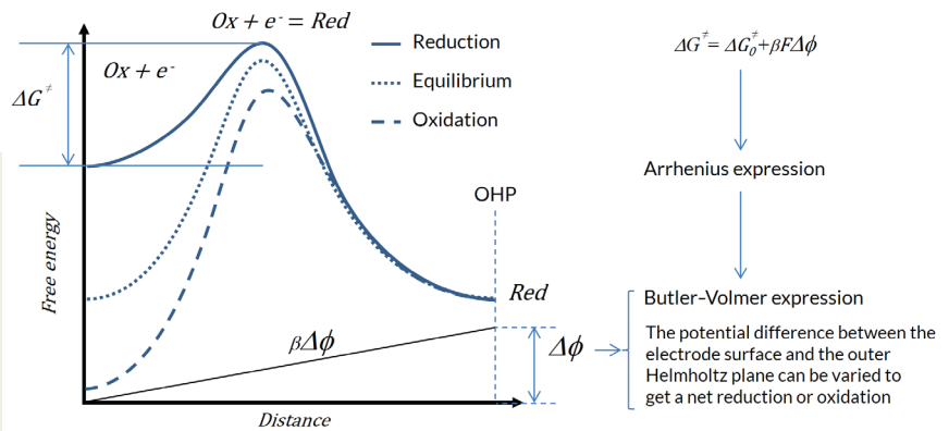
FIGURE 2. Depending on the electric potential at the metal surface, the surface can act as a cathode or as an anode. Connected to a more noble metal, a less noble metal surface acts as the anode. OHP denotes the outer Helmholtz plane of the charged double layer. Here, \beta denotes the symmetry factor, and F denotes the Faraday constant.
