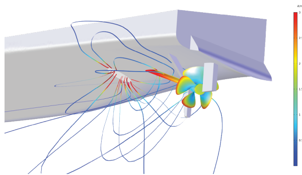
FIGURE 14. Streamlines in seawater around an anode with impressed current that protects the propeller in a large cargo vessel. The inner parts of the impeller blades are slightly less protected than the rest of the structure.
