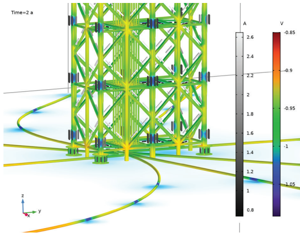
FIGURE 15. Potential distribution for an oil platform jacket structure and current output from the sacrificial anodes, two years after installation.
