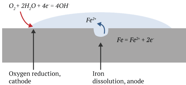
FIGURE 9. Corrosion may start due to uniform oxygen reduction and iron dissolution that eventually causes an oxygen gradient at the surface. This eventually gives a cathodic surface and an anodic surface; i.e., the reactions are no longer uniformly distributed.
