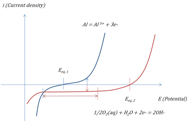
FIGURE 5. Oxygen reduction (red) is mass transport limited over a wide range of potential. The absolute negative current increases only at negative potential when hydrogen evolution starts.
