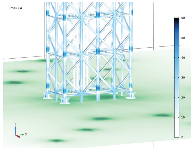
FIGURE 16. Deposited species in dimensionless units two years after installation of jacket structure. The deposited species affect the current distribution due to a reduced oxygen diffusion through the layer which reduces the amount of current passing through the surface.
