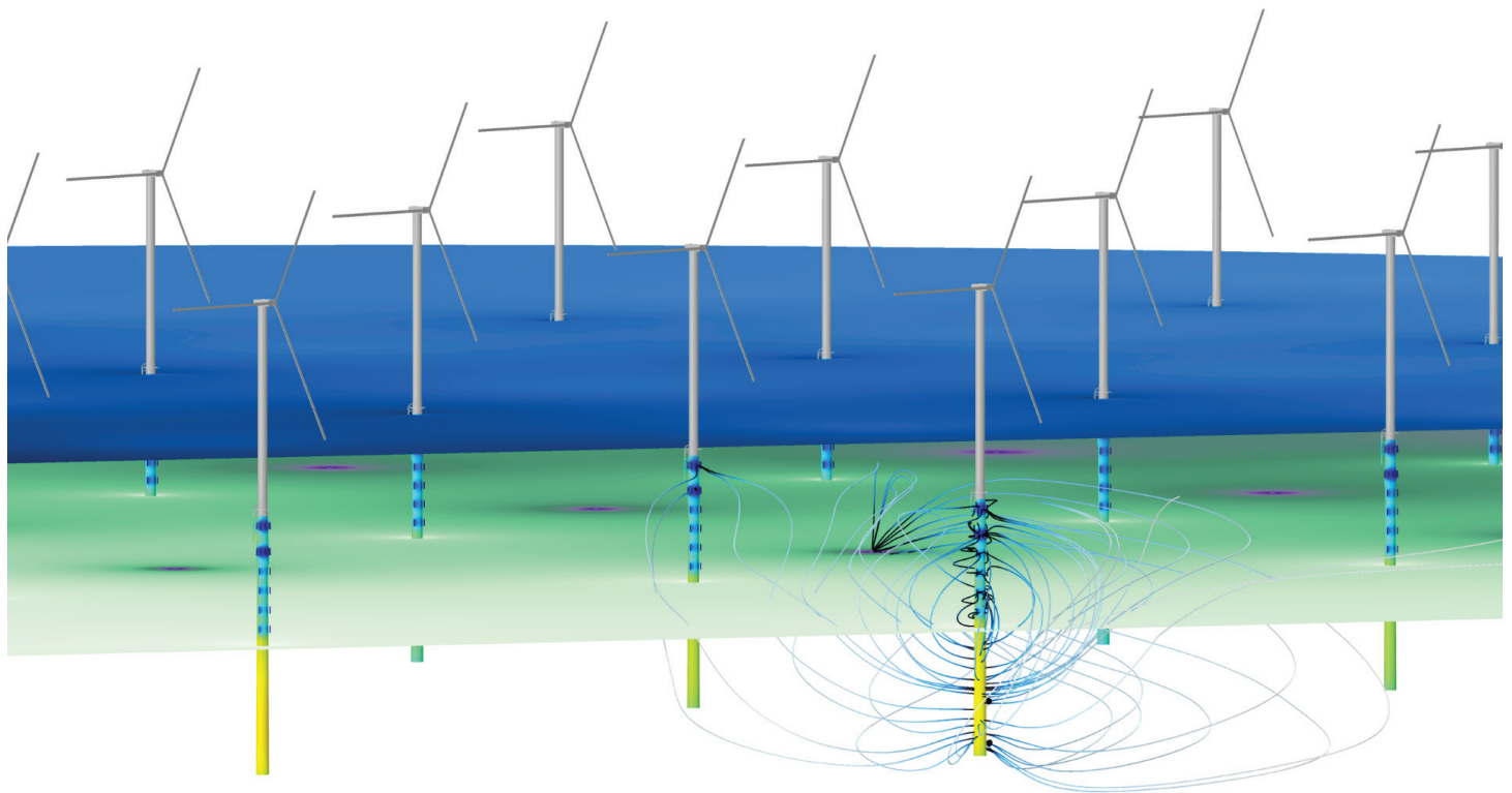
FIGURE 17. An offshore wind farm with parts of the structure below the sea surface is protected from corrosion using ICCP. The simulation is done with the purpose of positioning the anodes in order to protect the structure.
