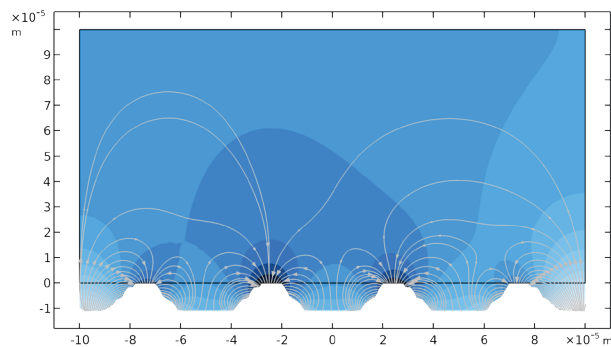
FIGURE 11. Results of a corrosion simulation using moving mesh. The initially flat surface starts to become slightly rugged after 60 h in contact with an electrolyte.
