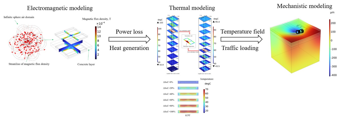
Figure 2 : Integrated Electro-Thermal-Mechanical Modeling
