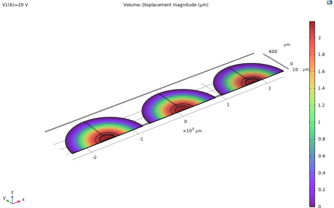
Figure 1 : FEM simulated the results of the micropump plate displacement in response to an applied voltage of 20V. Legend in \mu\text{m} . Max deflection approx. 2.2 \mu\text{m} .
