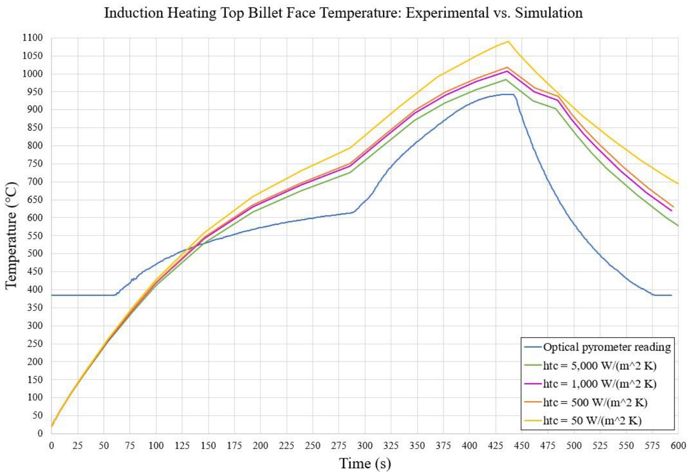
Figure 2 : Fig 2: Induction heating simulation results for varying effective heat transfer coefficients
