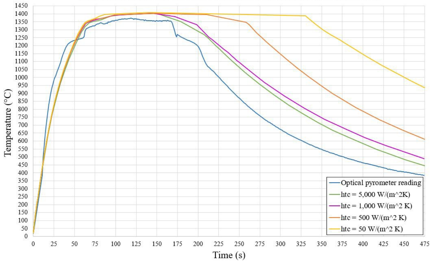
Figure 3 : Fig 3: Induction melting simulation results for varying effective heat transfer coefficients
