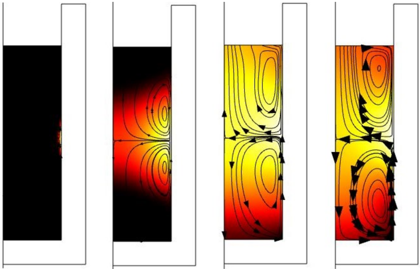
Figure 4 : Fig 4: Phase transition and electromagnetic stirring
