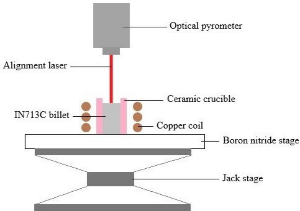
Figure 1 : Fig 1: Induction melting and optical pyrometer set-up
