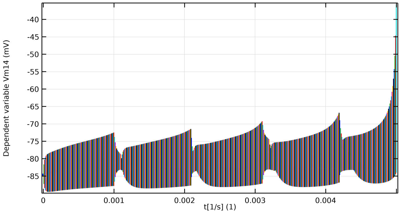
Figure 2 : Using 0.001 ms to examine nerve fiber membrane potential building over 5 wave periods until an action potential is generated.
