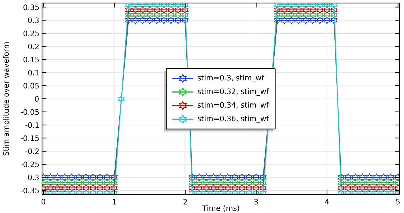
Figure 1 : Using 0.1 ms sampling rate to validate a charge-balanced rectangular waveform emitted by an electrode array on the human spinal cord to treat neuropathic pain.
