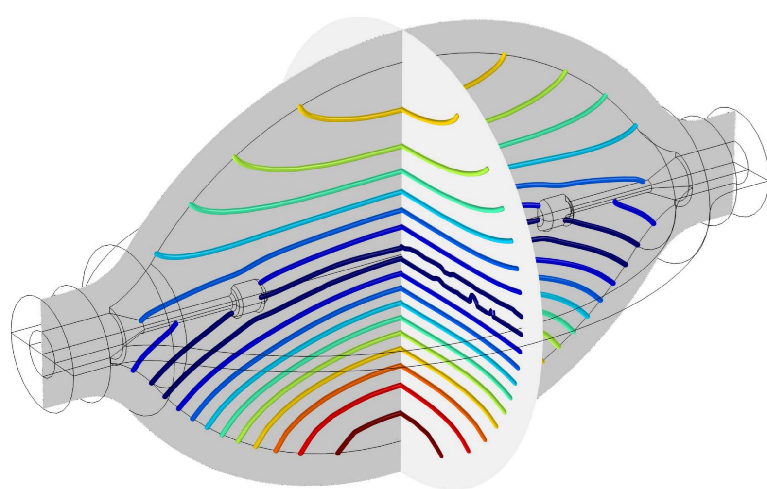
Figure 2. Lowest lying acoustic mode. Depicted is the absolute value of the acoustic pressure in arbitrary units.
