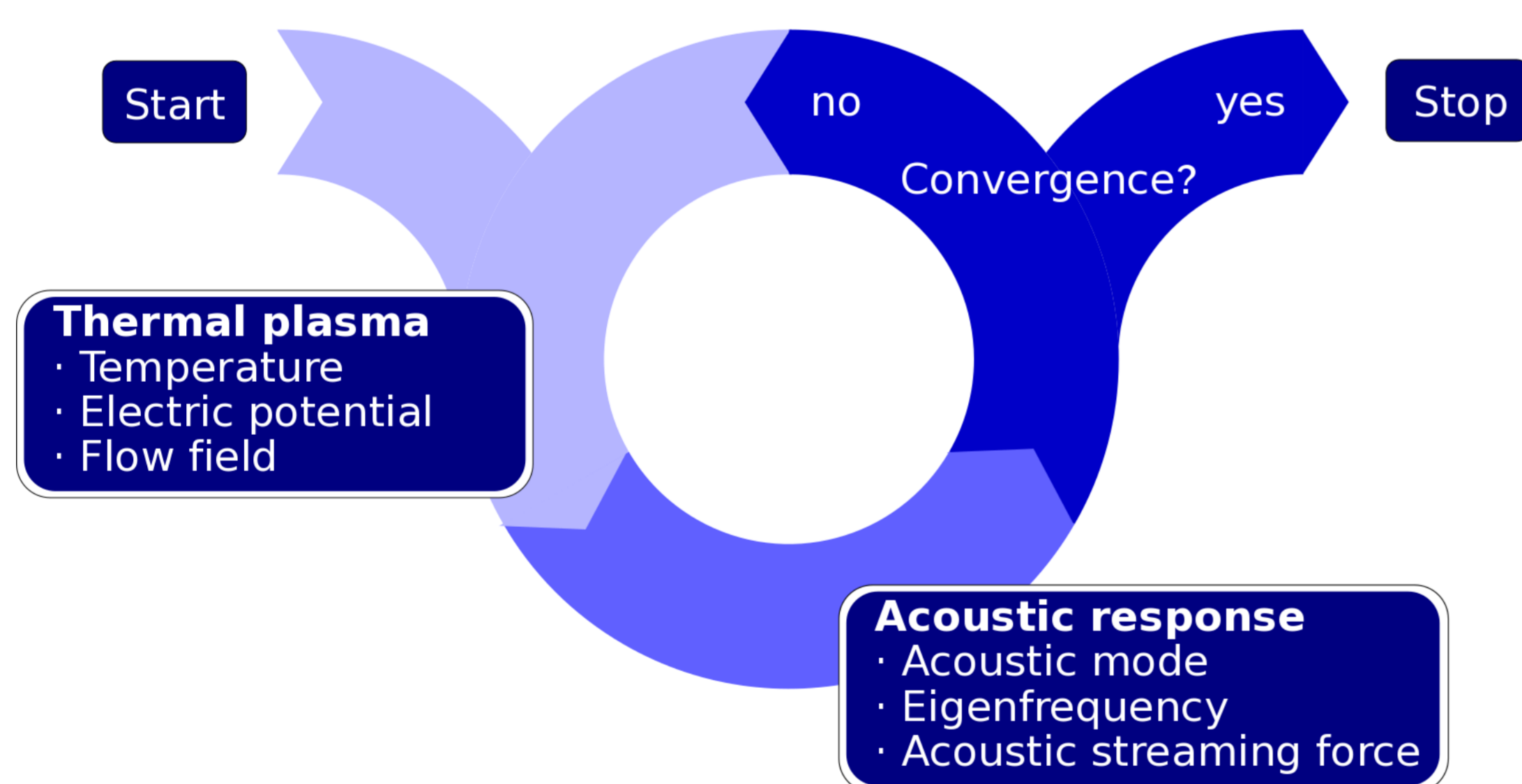
Figure 1. Recursion loop required for the coupling of plasma and acoustic model
