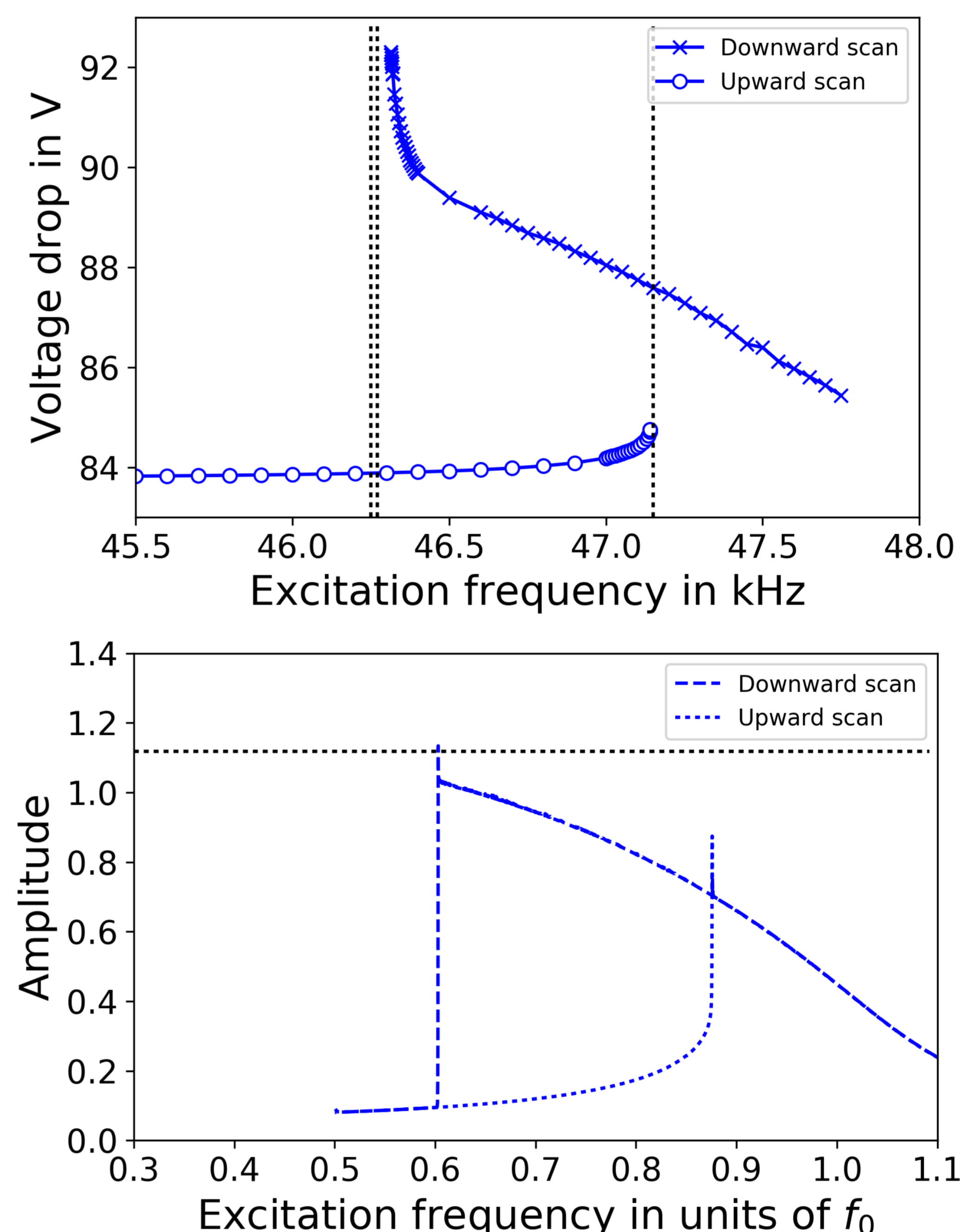
Figure 3. Voltage drop between electrodes (top) and response of Duffing oscillator (bottom)
